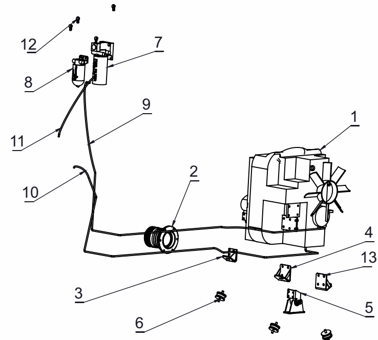
ENGINE ASSY (102 HP) 70720610
