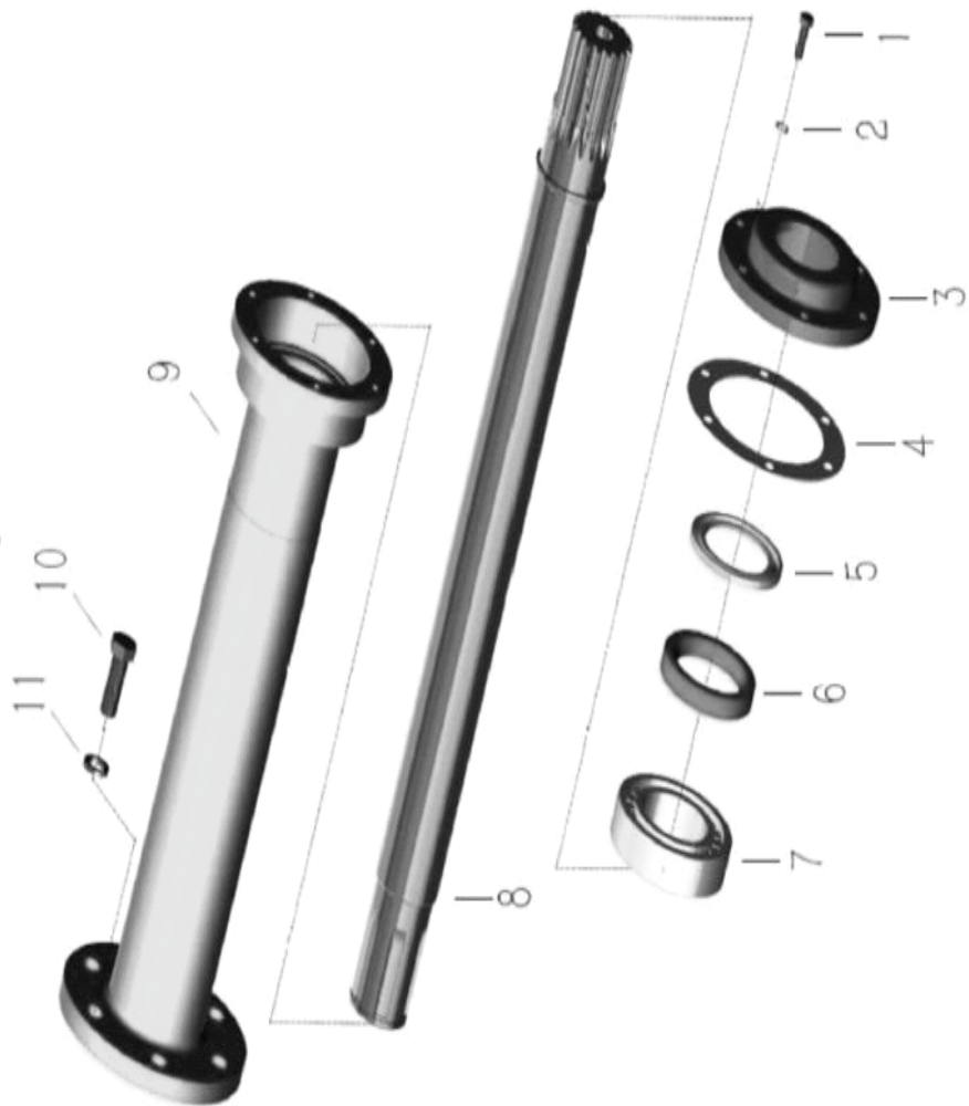
Gear Box Assy (HP) 10760491
